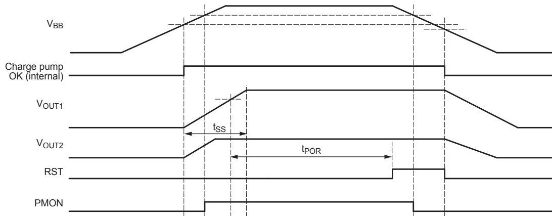
Normal Power-up Timing Diagram
