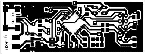
USBasp board optimized for homprew process
