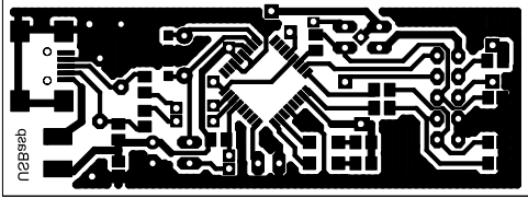
USBasp board optimized for homprew process
